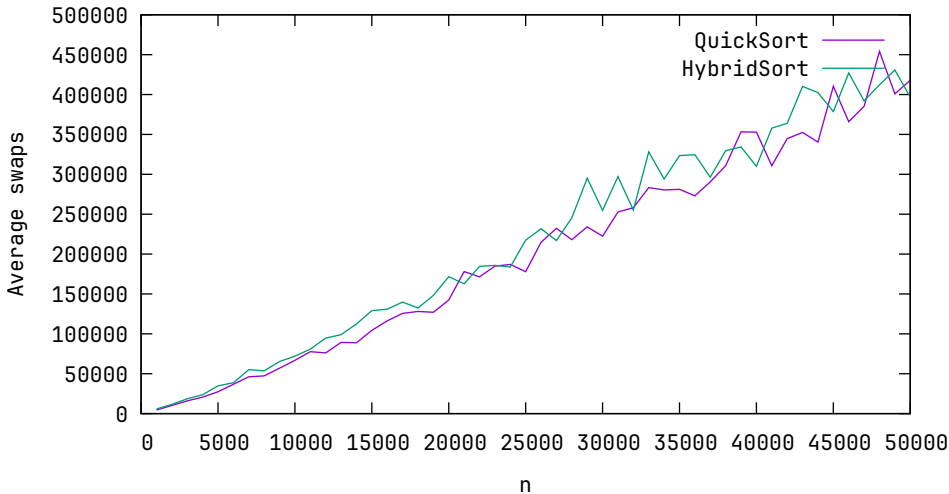
Average swaps, k = 1 , n \in 1000, 2000, \dots, 50000
