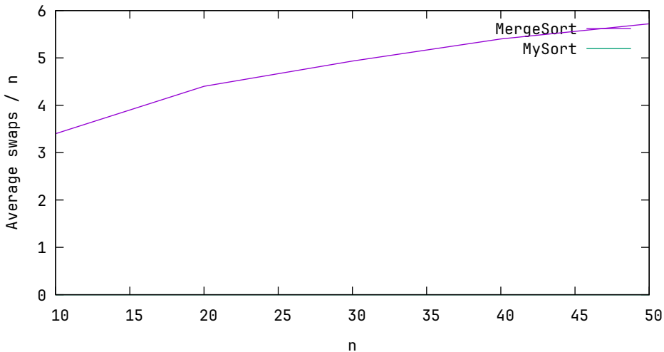
Average swaps / n, k = 10, n ∈ 10, 20, ..., 50
