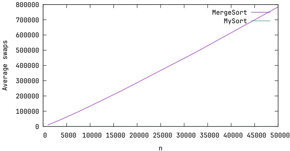
Average swaps, k = 100 , n \in 1000, 2000, \dots, 50000
