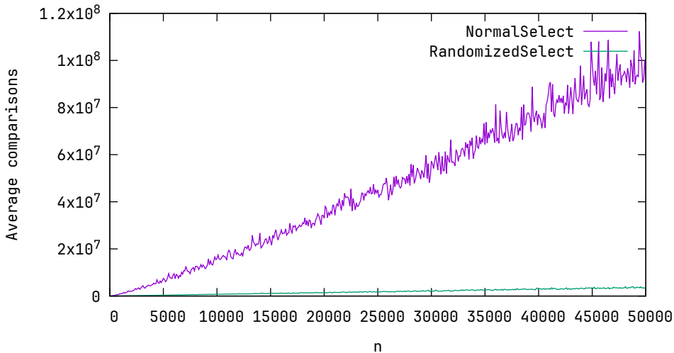
Average comparisons, k = 1 , n \in 100, 200, \dots, 50000
