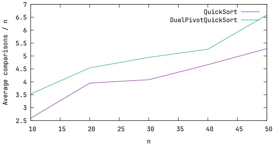
Average comparisons / n , k = 10 , n \in 10, 20, \dots, 50
