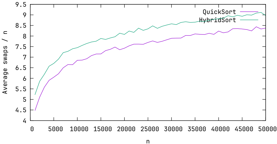
Average swaps / n, k = 100, n ∈ 1000, 2000, ..., 50000
