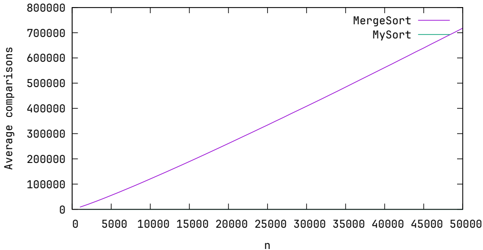
Average comparisons, k = 1 , n \in 1000, 2000, \dots, 50000
