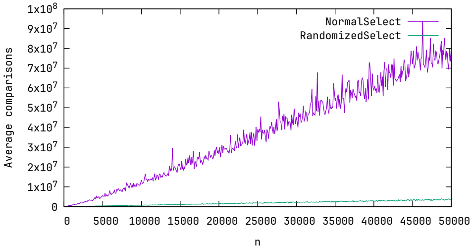
Average comparisons, k = n , n \in 100, 200, \dots, 50000
