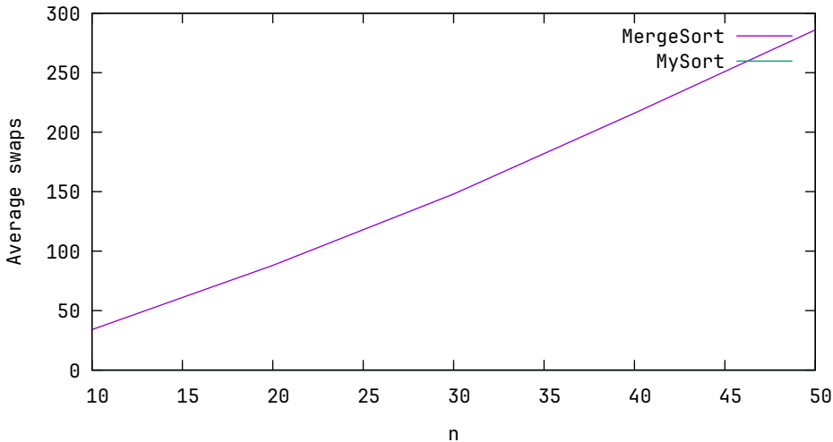
Average swaps, k = 10 , n \in 10, 20, \dots, 50
