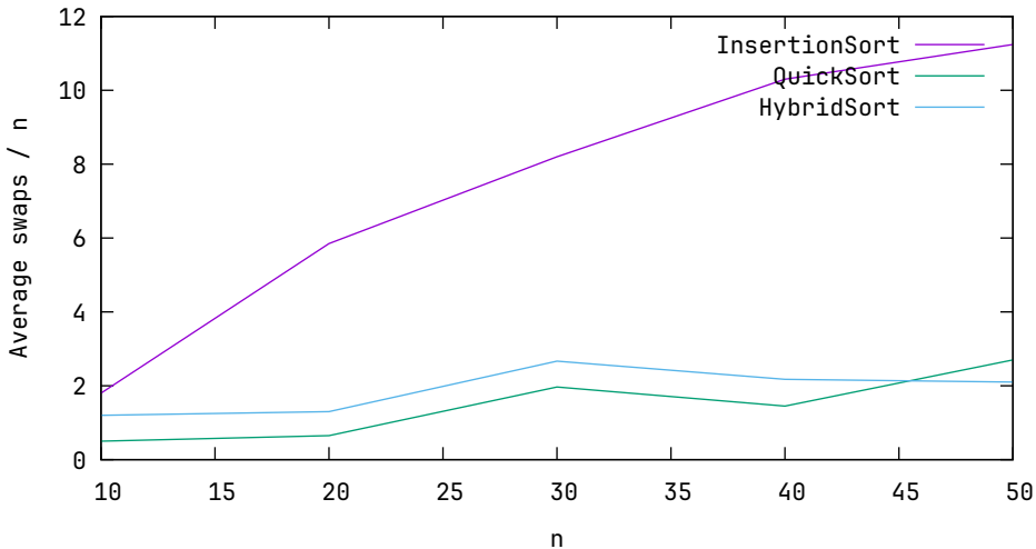
Average swaps / n, k = 1, n ∈ 10, 20, ..., 50
