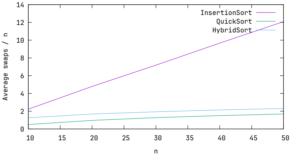
Average swaps / n, k = 100, n ∈ 10, 20, ..., 50
