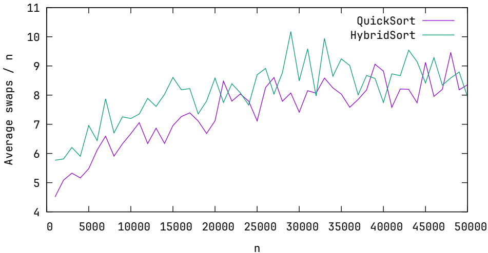
Average swaps / n, k = 1, n ∈ 1000, 2000, ..., 50000
