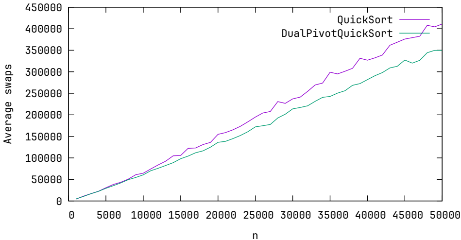
Average swaps, k = 10 , n \in 1000, 2000, \dots, 50000
