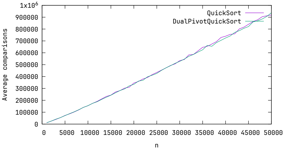
Average comparisons, k = 10 , n \in 1000, 2000, \dots, 50000
