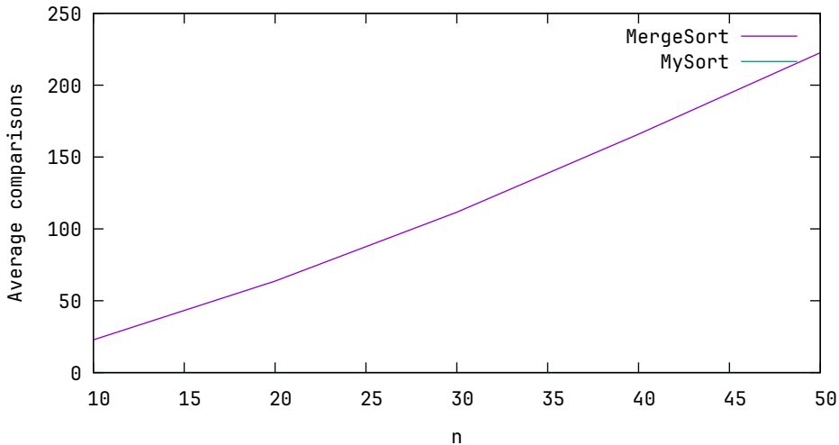
Average comparisons, k = 100 , n \in 10, 20, \dots, 50
