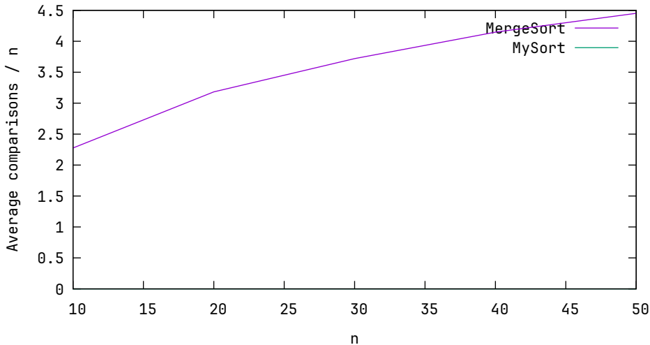
Average comparisons / n, k = 100, n ∈ 10, 20, ..., 50
