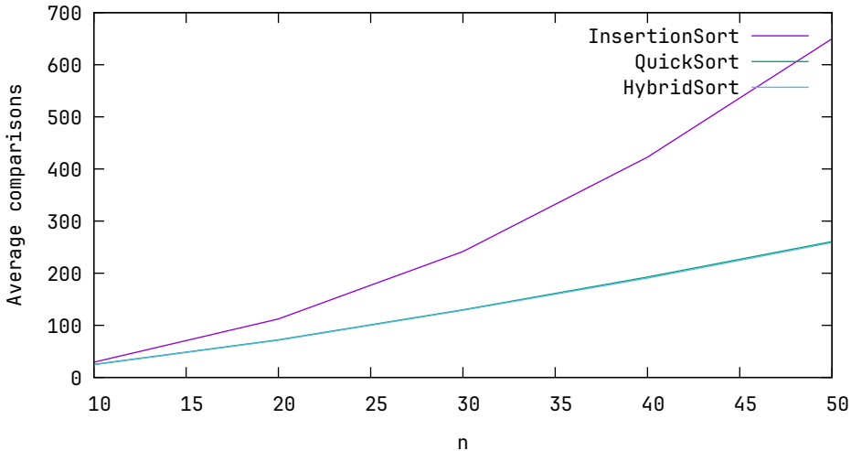
Average comparisons, k = 100 , n \in 1000, 2000, \dots, 50000
