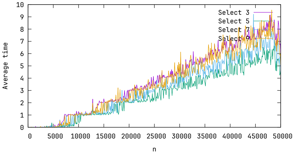
Average time, n \in 100, 200, \dots, 50000
