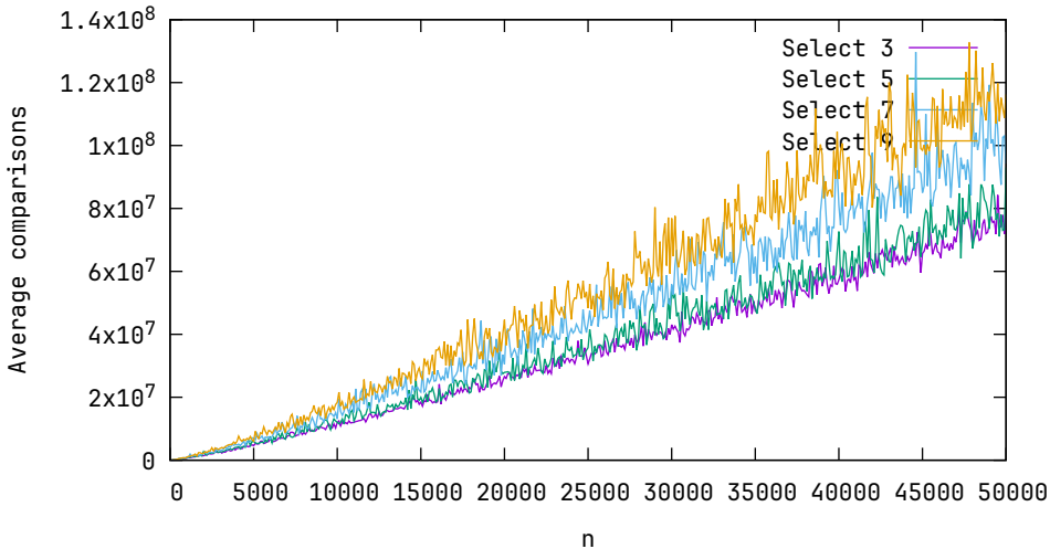
Average comparisons, n \in 100, 200, \dots, 50000
