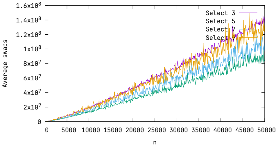
Average swaps, n \in 100, 200, \dots, 50000
