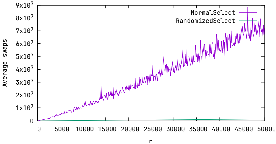
Average swaps, k = n , n \in 100, 200, \dots, 50000
