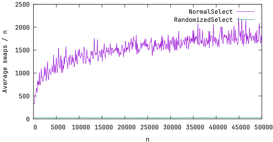
Average swaps / n, k = 1, n ∈ 100, 200, ..., 50000
