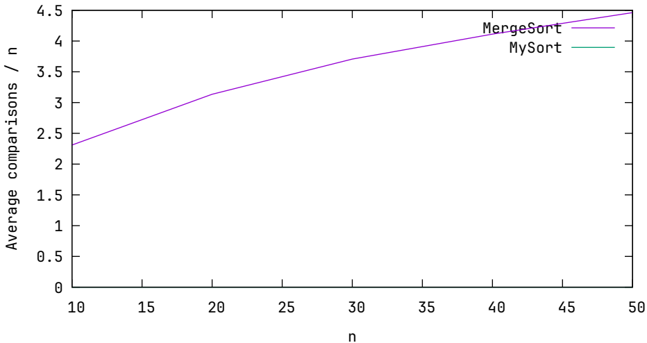
Average comparisons / n, k = 10, n ∈ 10, 20, ..., 50
