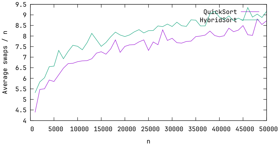
Average swaps / n, k = 10, n ∈ 1000, 2000, ..., 50000
