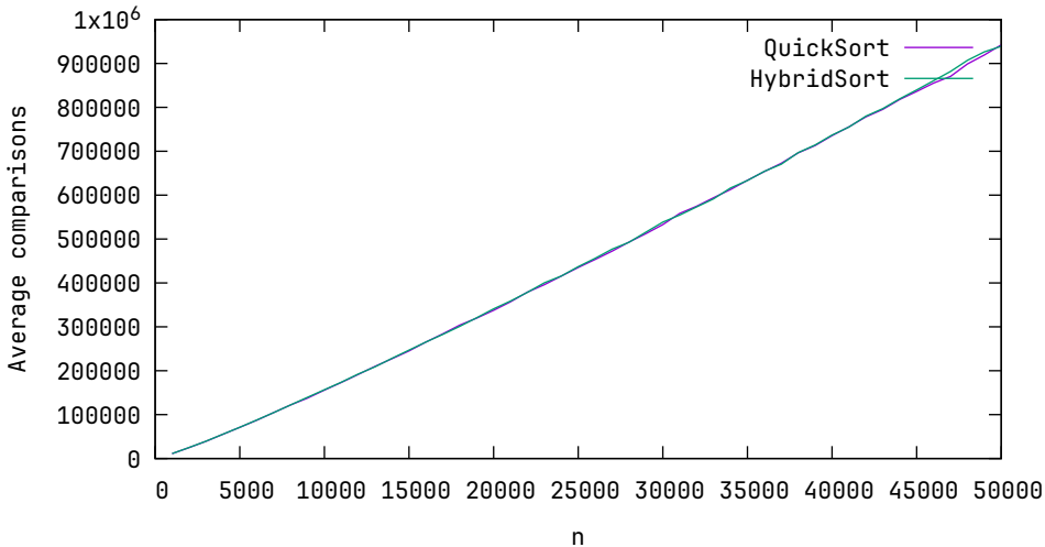
Average comparisons, k = 100 , n \in 1000, 2000, \dots, 50000
